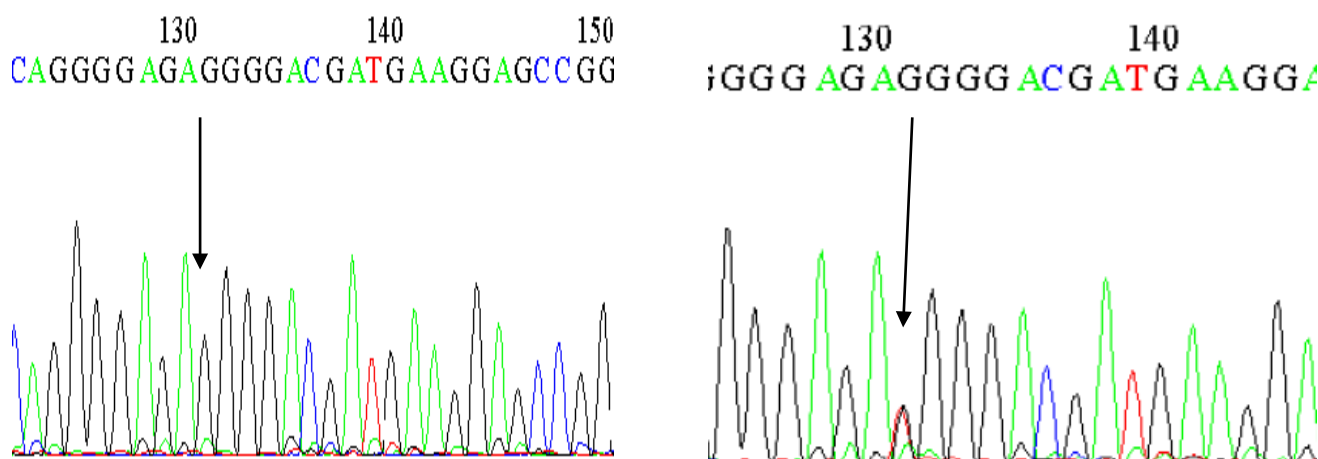
Figure 5: Nucleotide sequence chromatogram representing two does genotype of BCL-2 (-938C>A) gene. The left figure is a GG homozygote, and the right figure is a G/T heterozygote.
