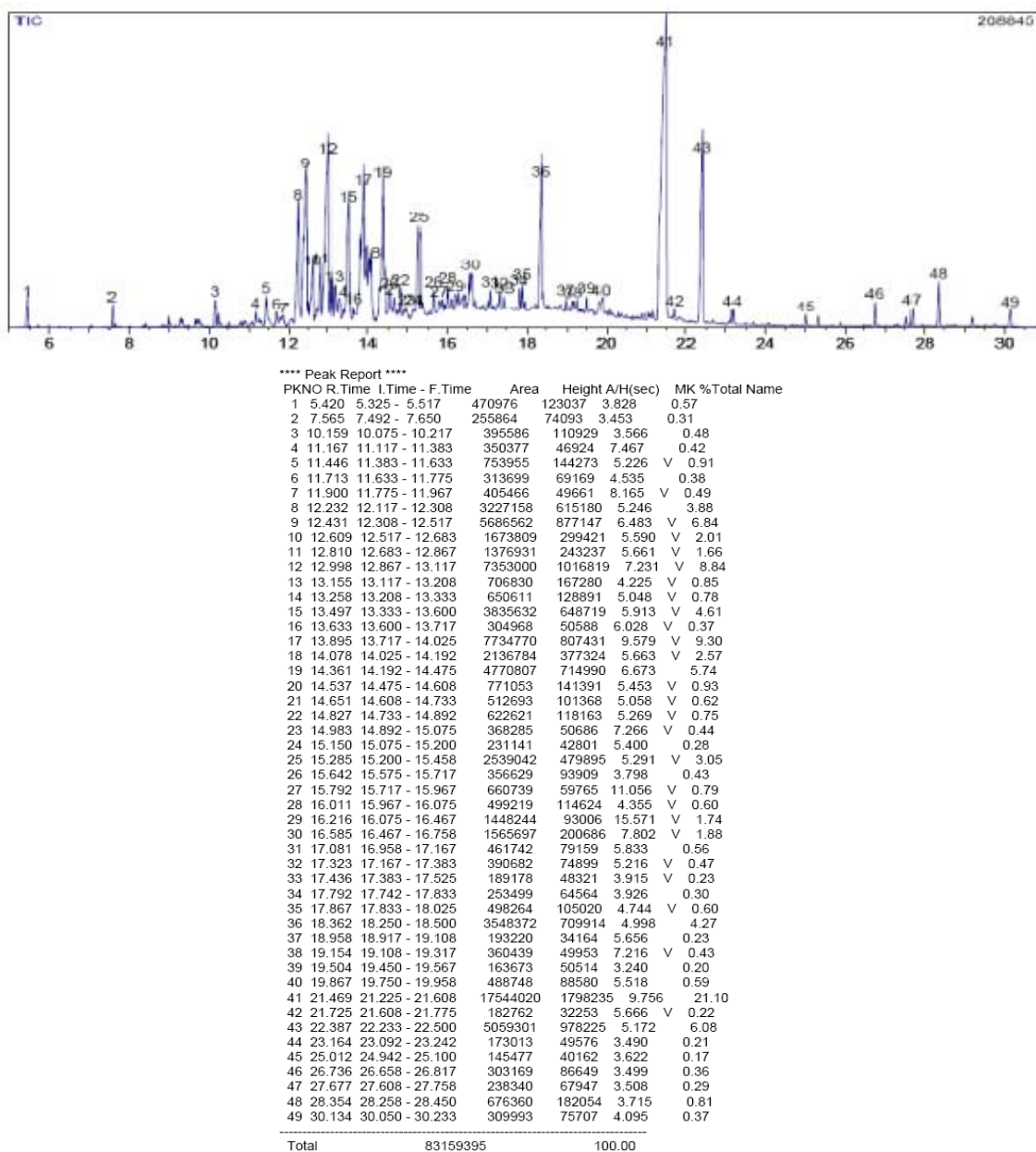
Figure 1. GC-MS results of the essential oil of iler leaf
