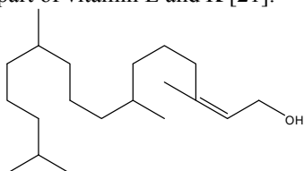
Figure 2 Structure of phytol
